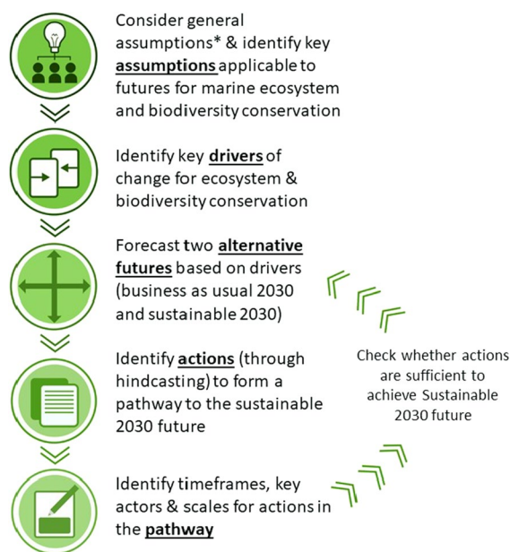
Fig. 1 An overview of the methods followed to develop alternative scenarios of 2030 for marine ecosystem and biodiversity conservation (* from Nash et al. 2021a, this issue)
